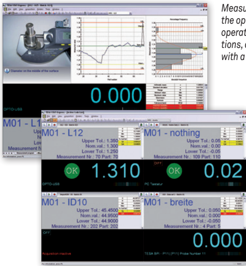
Simultaneous data acquisition from several measurement programmes
