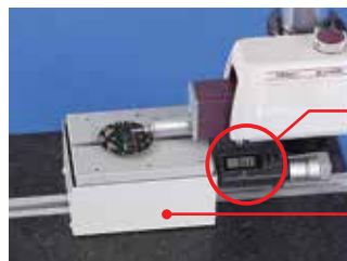
DAT screen guides the user when leveling Digimatic micrometer head Amount of micrometer head adjustment required Leveling table (DAT) (Option)
