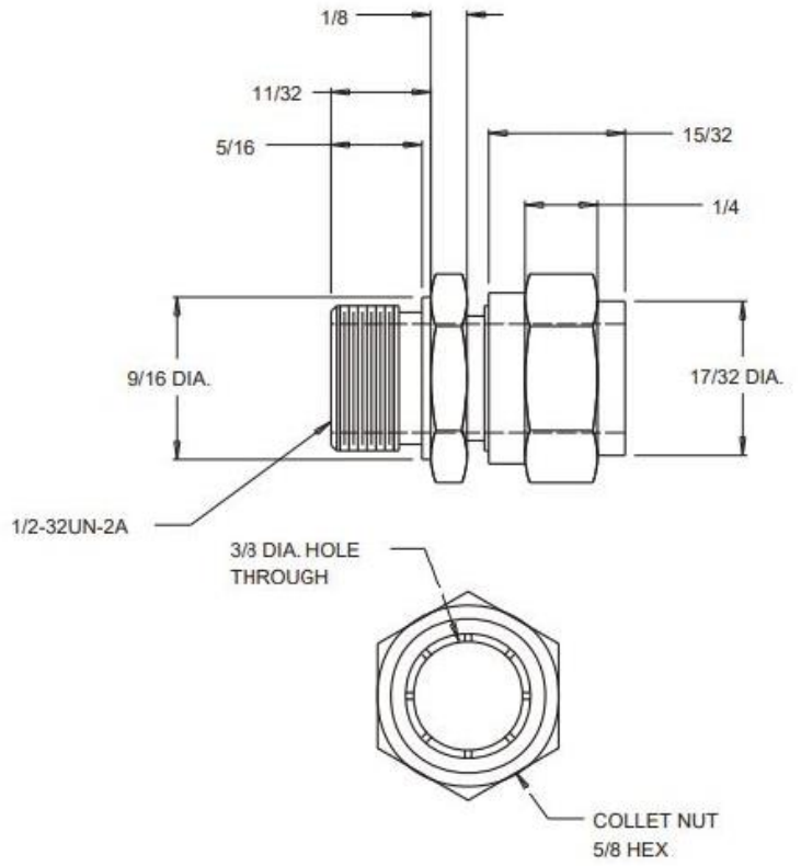
MOUNTING COLLET, CDI98
