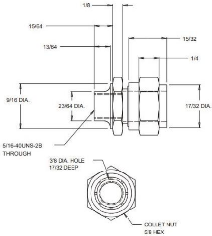
MOUNTING COLLET, CDI92
