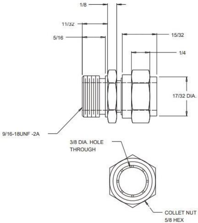
MOUNTING COLLET, CDI96
