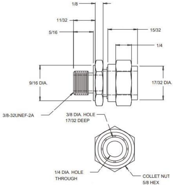
MOUNTING COLLET, CDI98
